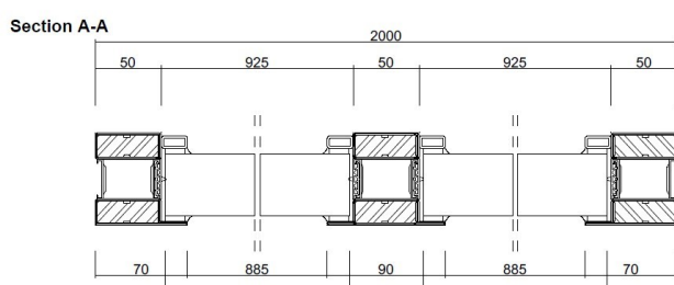
Typical standard profile
