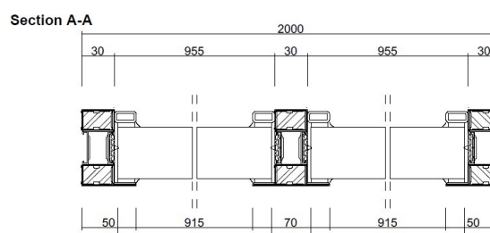
Typical slimline profile
