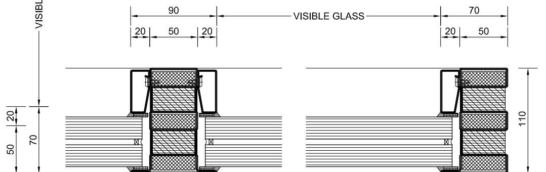
TYPICAL HORIZONTAL SECTION
