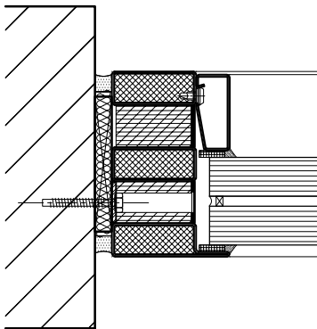
MASONRY WALL
