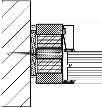
MASONRY WALL
