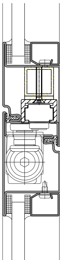
FULLY CONCEALED DORMA ITS-96 CLOSER
