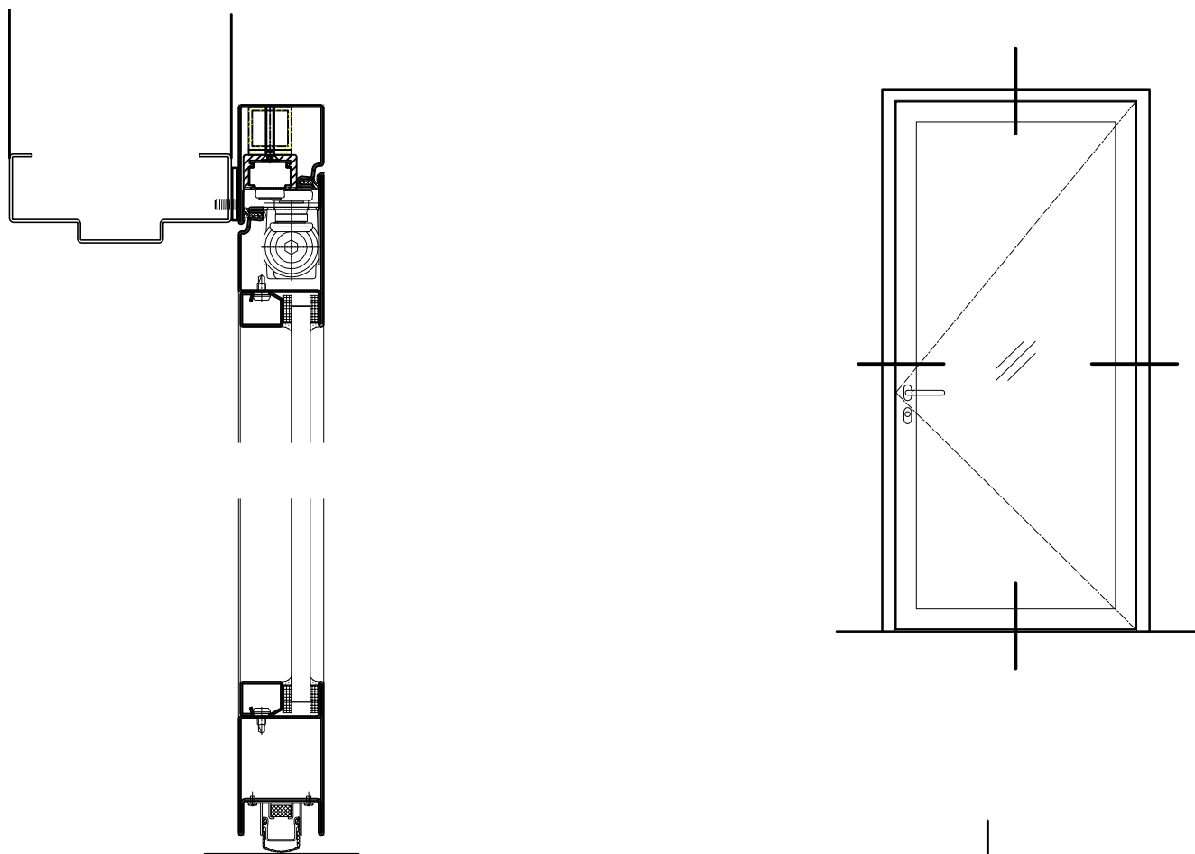
TYPICAL VERTICAL SECTION
