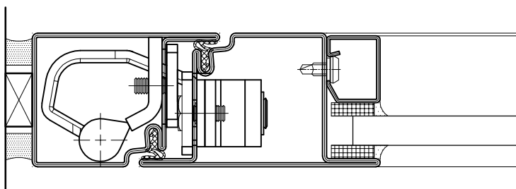
FULLY CONCEALED FORSTER HINGE 917611
