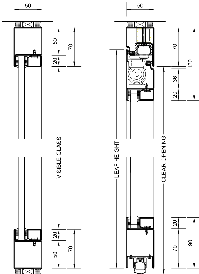
TYPICAL VERTICAL SECTION A - A
