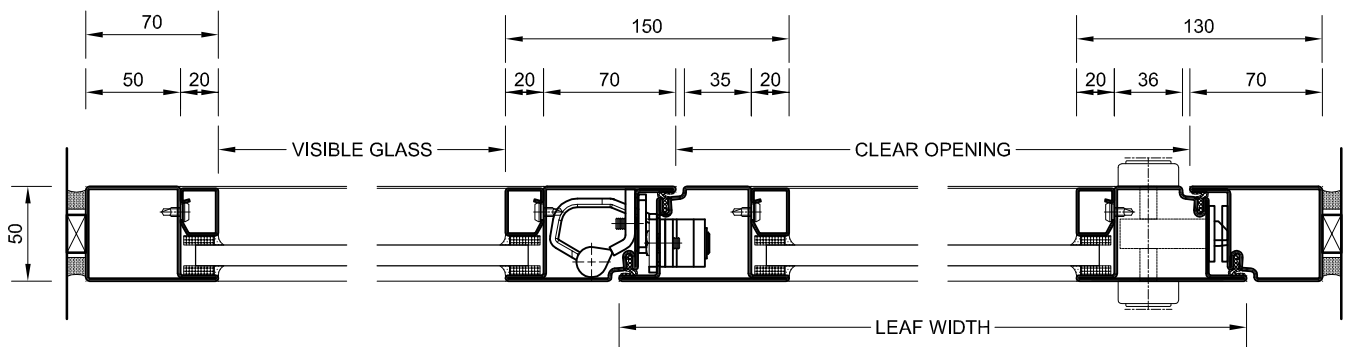
TYPICAL HORIZONTAL SECTION C - C
