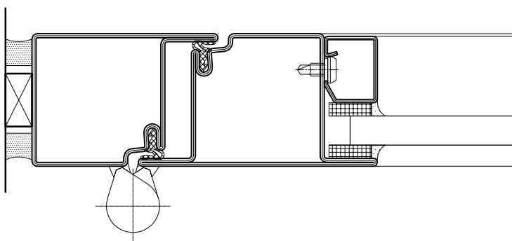
WELD ON FORSTER HINGE 907662
