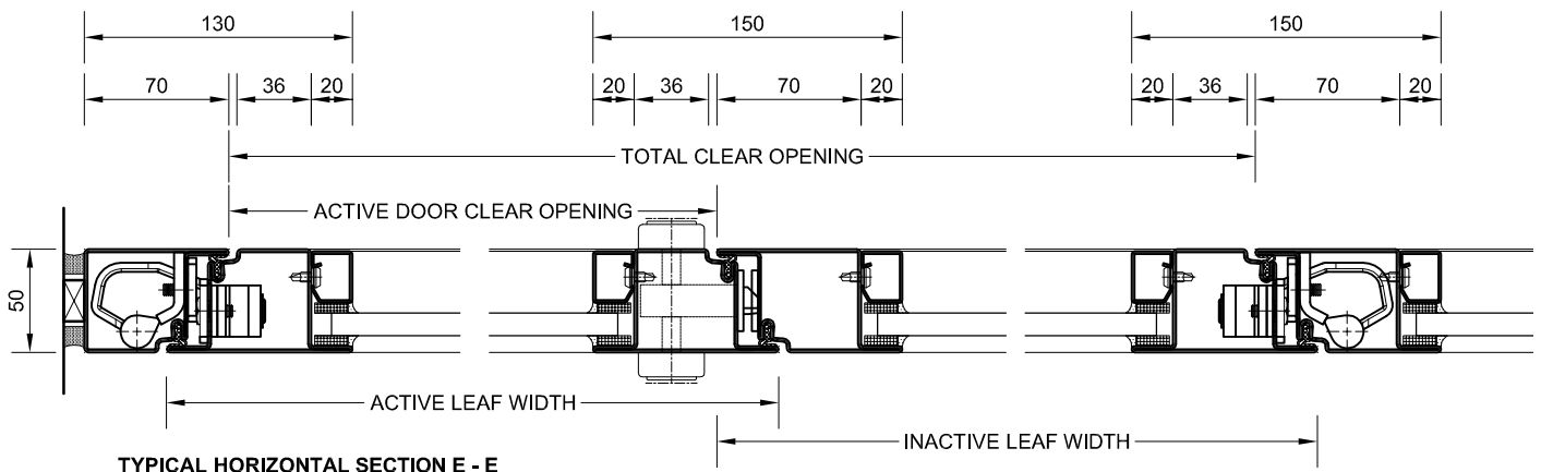
TYPICAL HORIZONTAL SECTION E - E
