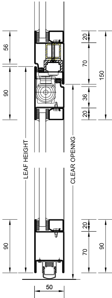
TYPICAL VERTICAL SECTION D - D
