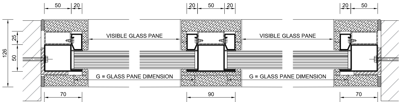
PRESTO TYPICAL SECTION - WITH IN THE SLAB
